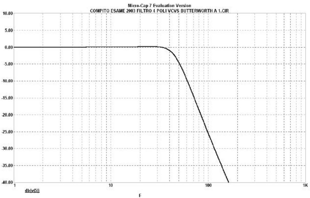
FILTRO 4 POLI VCVS BUTTERWORTH F=40HZ A0=1
