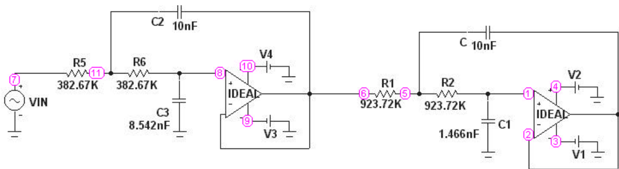
FILTRO 4 POLI VCVS BUTTERWORTH F=40HZ A0=1
